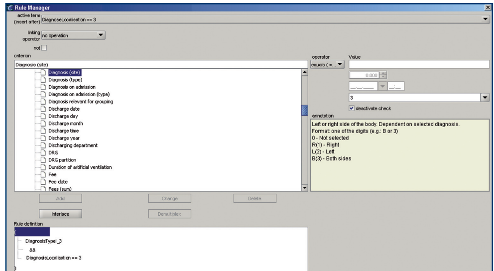
Rule manager
